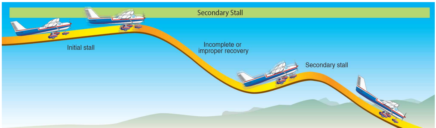
Figure 5-13. Secondary stall.
