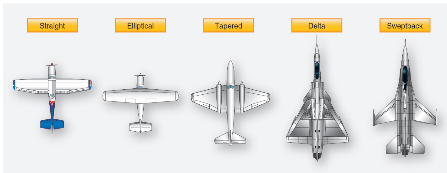
Figure 12-1. Airfoil types.
