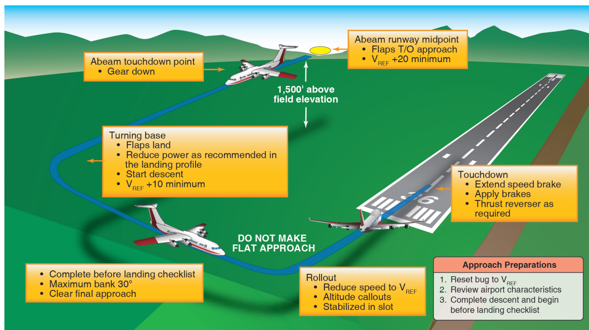
Figure 16-17. Typical approach and landing profile.
