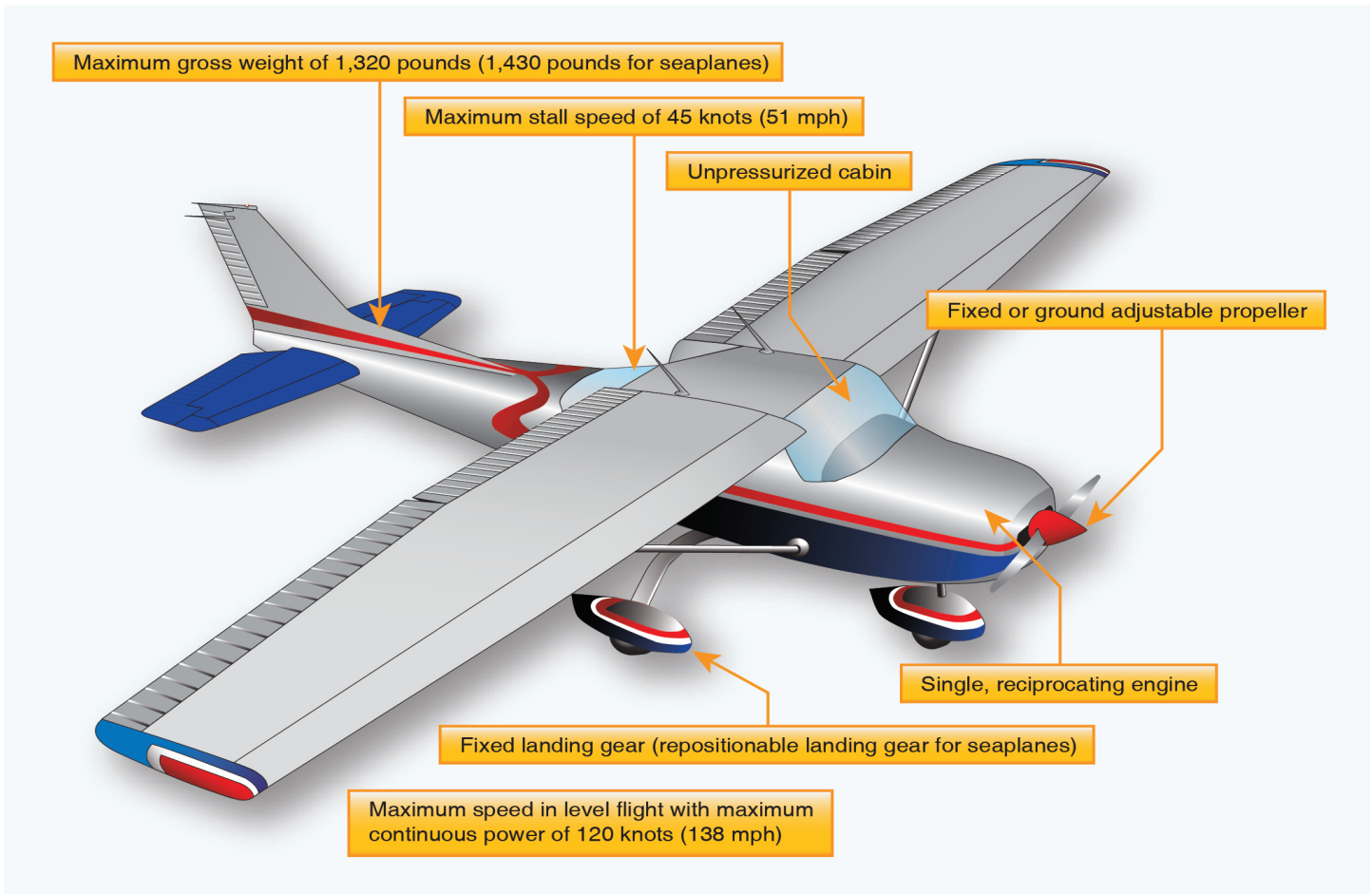
Figure 17-2. Light-sport airplane.
