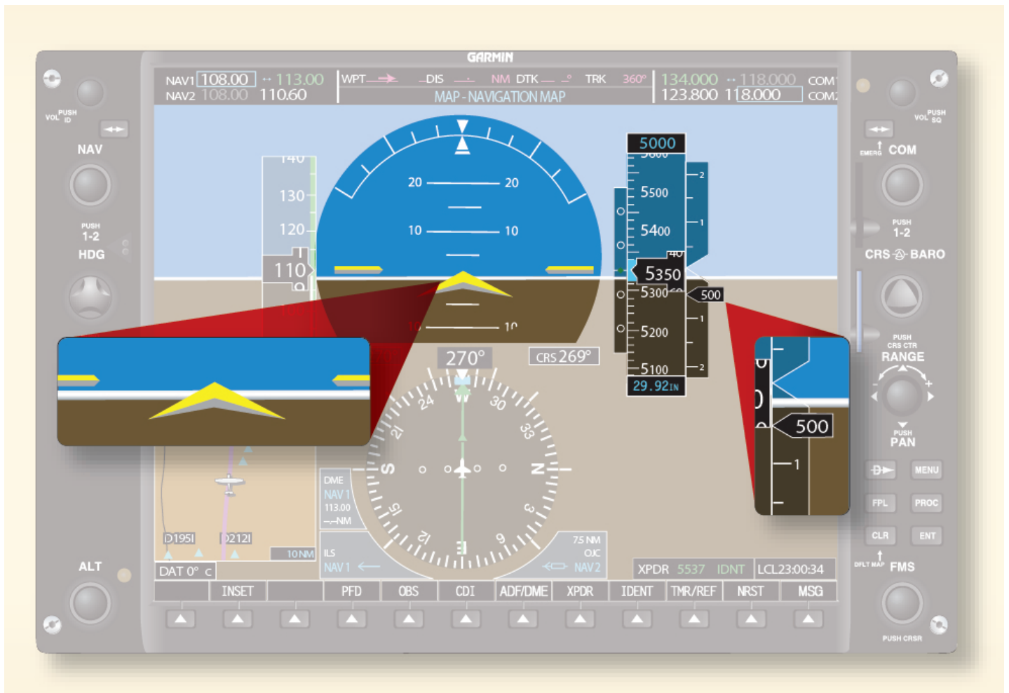
Figure 18-14. Level climb.
