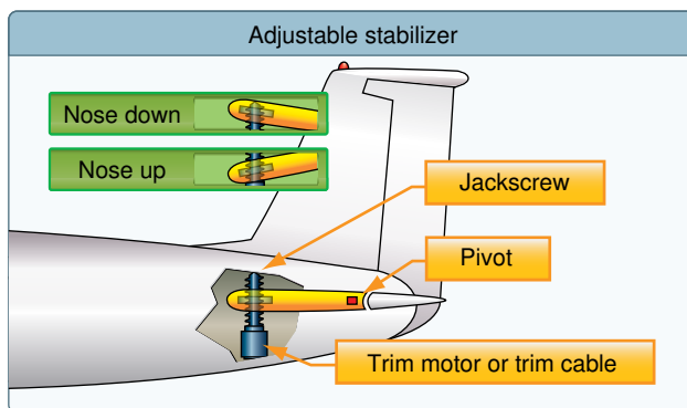
Figure 6-23. Some aircraft, including most jet transports, use an adjustable stabilizer to provide the required pitch trim forces.
