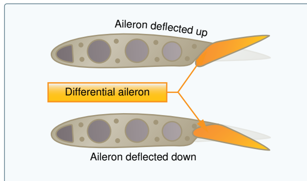
Figure 6-6. Differential ailerons.
