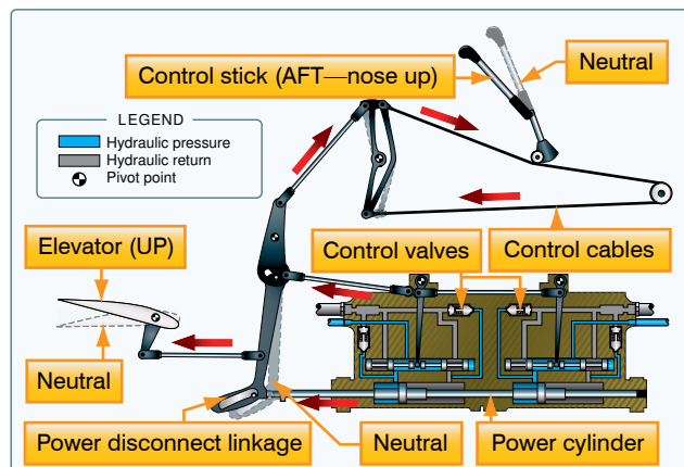
Figure 6-2. Hydromechanical flight control system.
