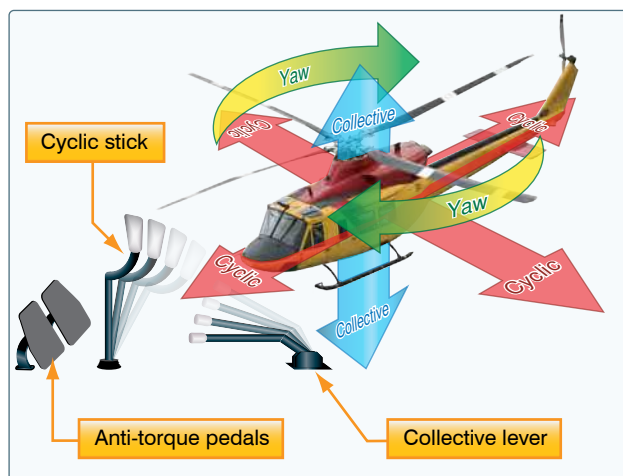
Figure 6-3. Helicopter flight control system.
