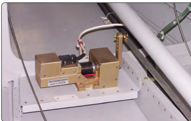
Figure 6-24. Basic autopilot system integrated into the flight control system.
