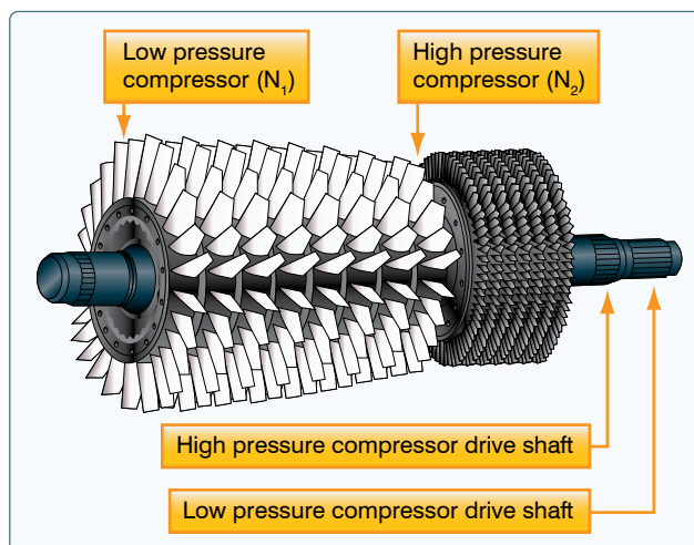
Figure 7-27. Dual-spool axial-flow compressor.
