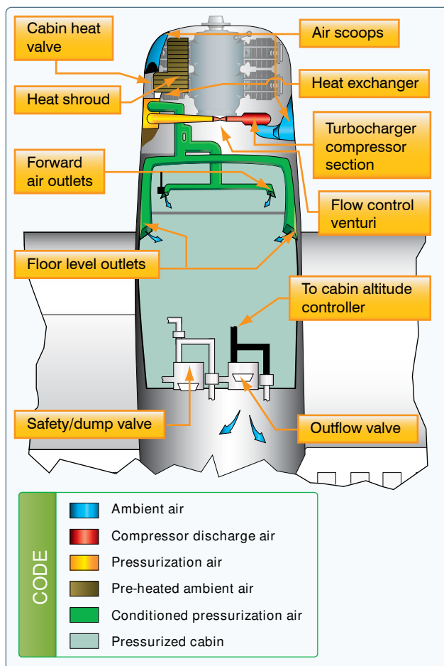
Figure 7-40. High performance airplane pressurization system.
