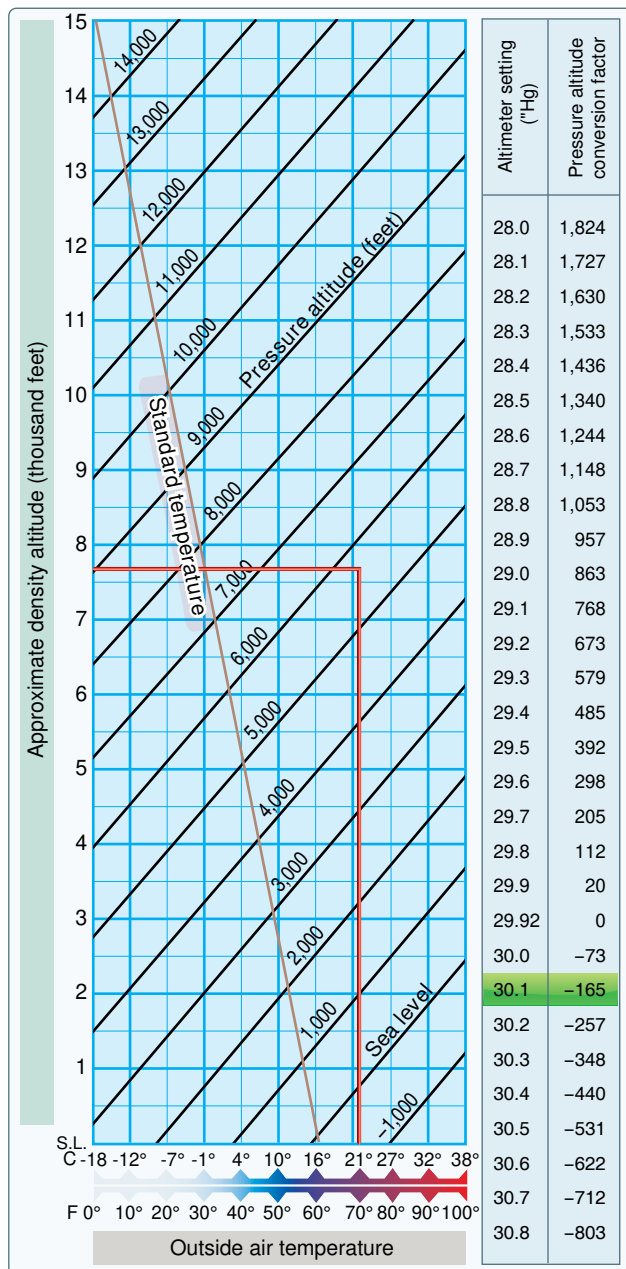
Figure 11-22. Density altitude chart.
