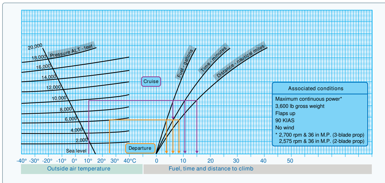
Figure 11-25. Fuel, time, and distance climb chart.
