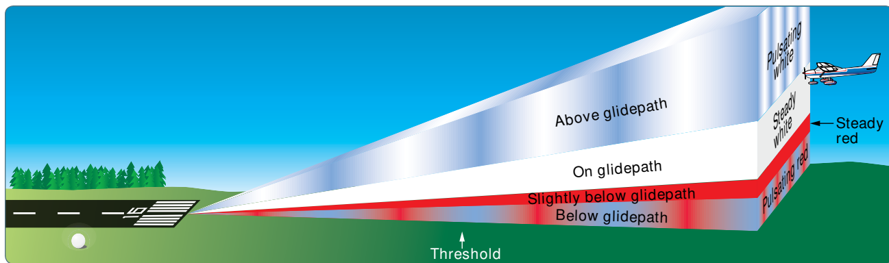
Figure 14-32. Pulsating visual approach slope indicator.
