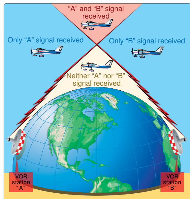
Figure 16-28. VHF transmissions follow a line-of-sight course.
