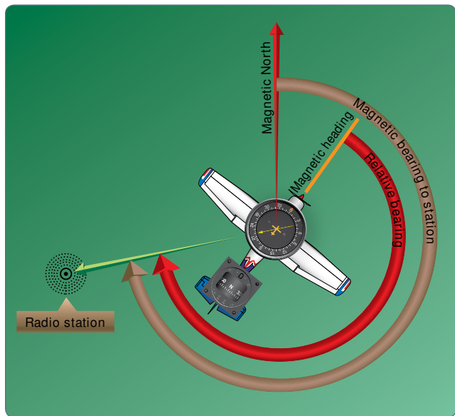
Figure 16-38. ADF terms.
