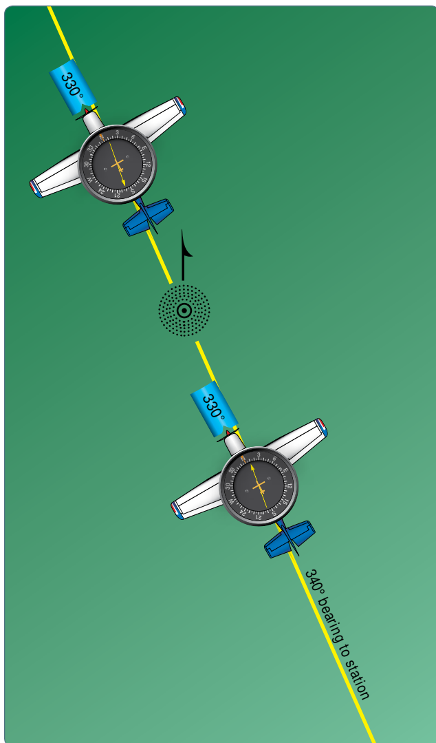
Figure 16-39. ADF tracking.
